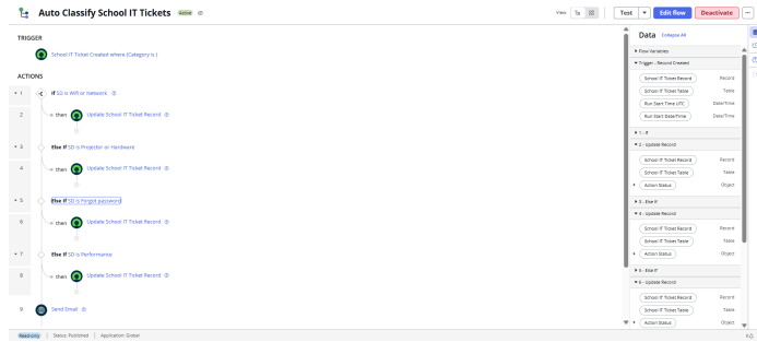
Figure 2: Flow Designer implementation of the automatic classification requirement.
